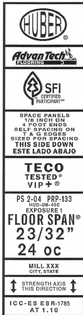
FIGURE 1—TYPICAL PANEL GRADE STAMP
